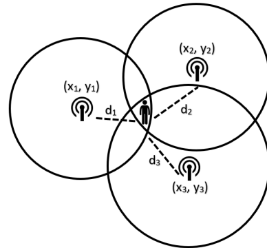
Fig. 7: Trilateration method. The user location is inferred as the intersection of the nearest beacons using geometry.
