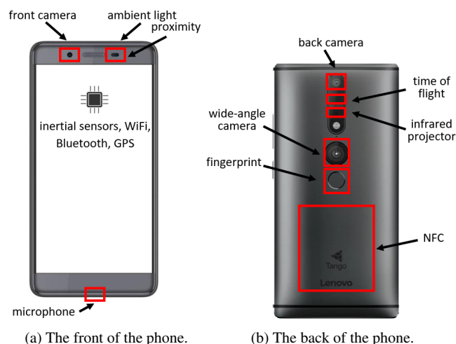
Fig. 3: Relative position of most smartphones sensors, illustrated on our Lenovo Phab 2 test phone. Some sensors are embedded within the phone, while others are exposed. The battery occupies the majority of space at the bottom half of the phone.
