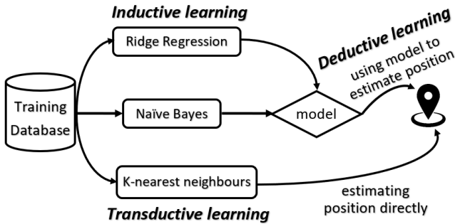
Fig. 9: The machine learning approaches for fingerprinting.
