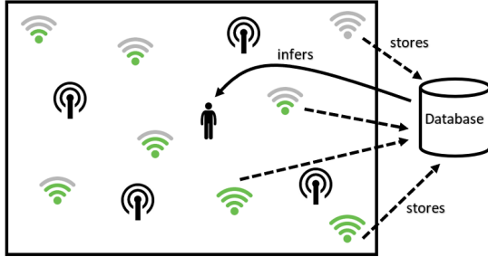
Fig. 8: Fingerprinting method.
