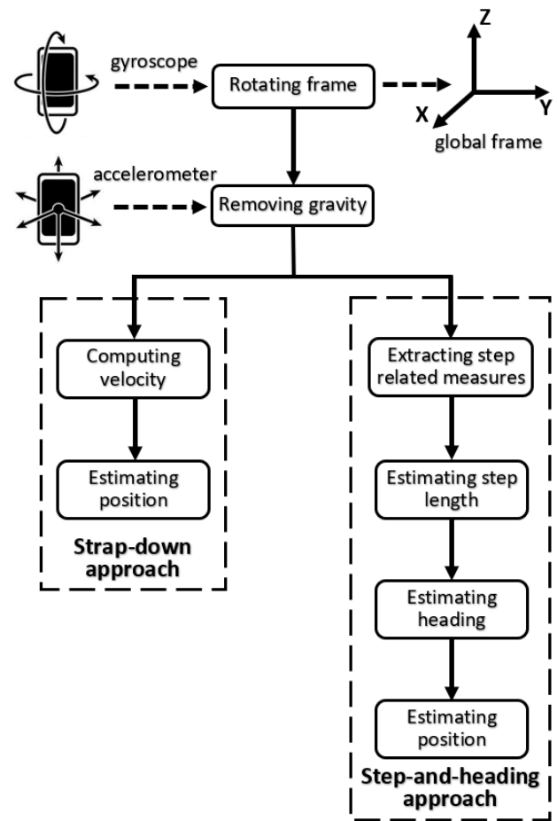
Fig. 13: The two main approaches for inertial based system.
