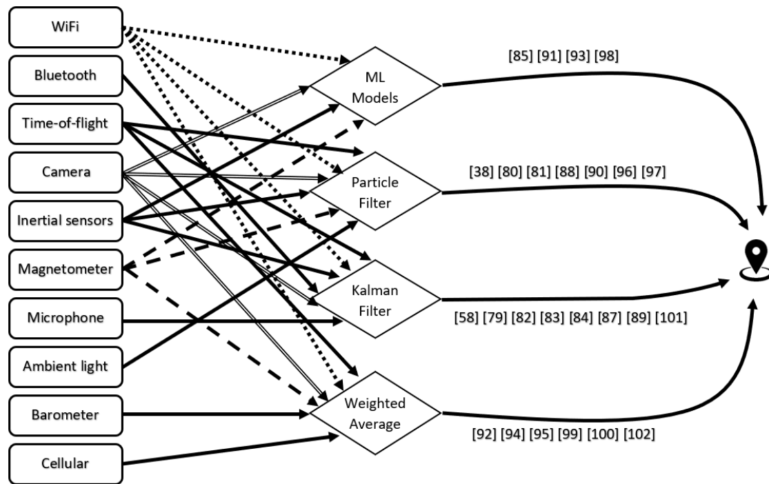
Fig. 15: Combination of smartphones sensors with respect to the data fusion methods. Different styles of arrows are used to distinguish amongst sensor types and how they combine.
