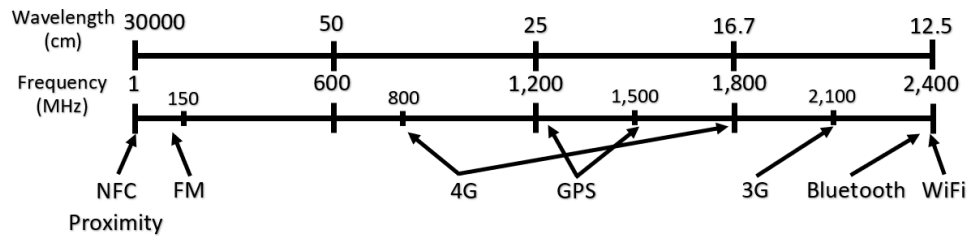
Fig. 4: The electromagnetic spectrum.
