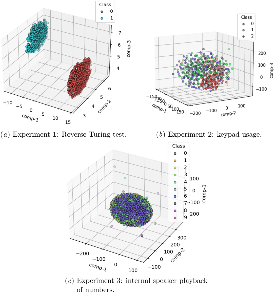
Figure 3: Dimensionality reduction of magnetometer changes.
